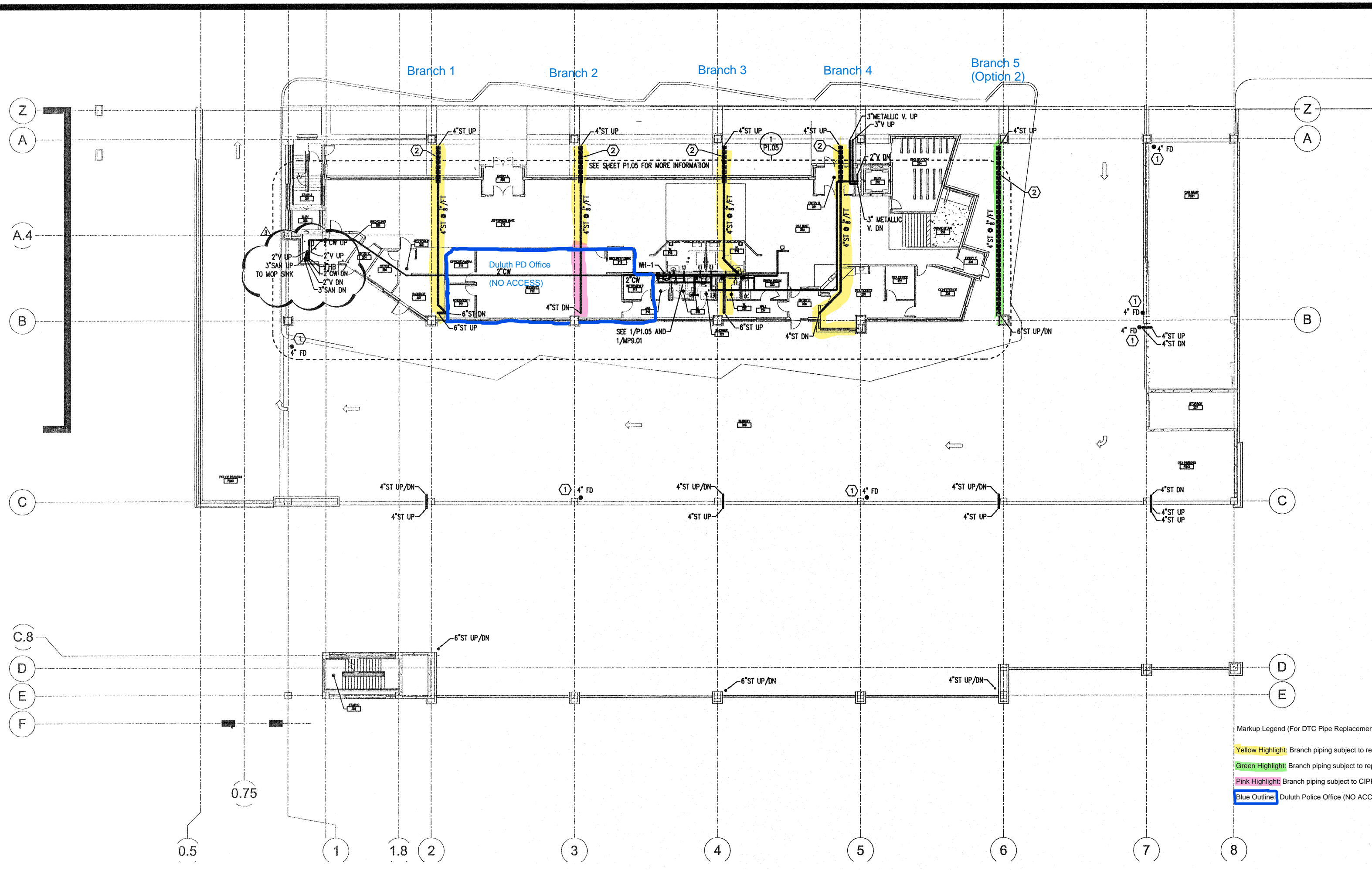
1 P1.02 LEVEL 2 PLUMBING PLAN 1/16" = 1'-0"
