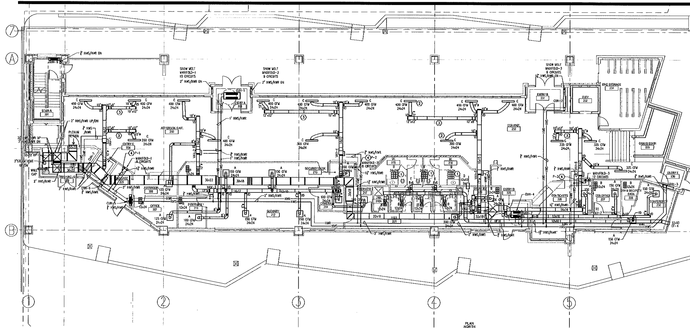
1 ENLARGED TRANSIT CENTER HVAC PLAN 1/8" = 1'-0" PLAN NORTH
