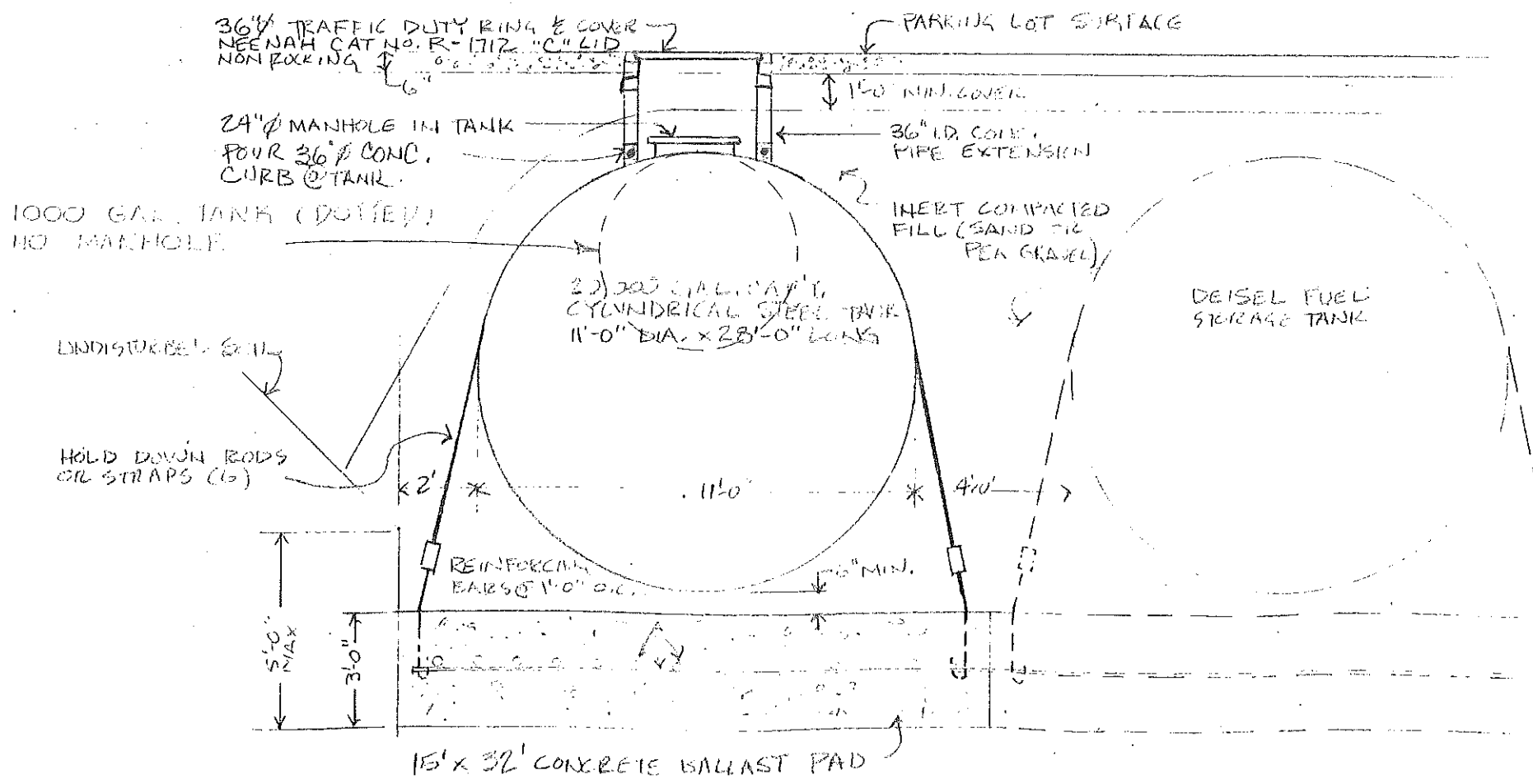
1/M3 UNDERGROUND FUEL OIL STORAGE TANK
